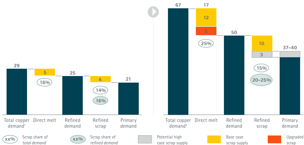
Copper Demand, 2018 Million Tonnes
